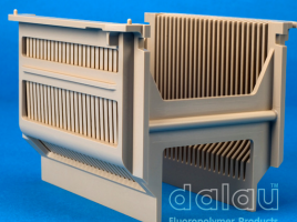
Wafer Carrier, PEEK 25 slots
